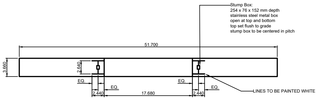
WICKET LAYOUT
